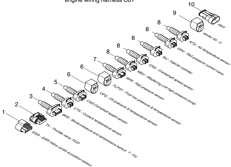
engine wiring harness C81
